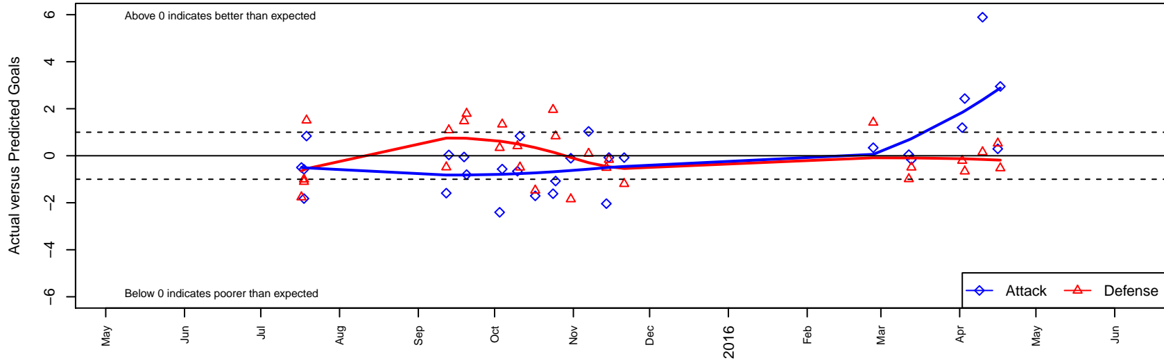
HSC Boca B04 Dots are actual minus expected GF (blue circles) and GA (red triangles). Blue line is smoothed change in attack strength. Red is smoothed change in defense strength.
